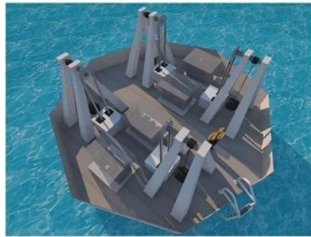
Figure 3. A Device for Generating Sea Wave Electricity from A Pendulum
