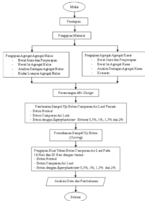
25 Gambar 1. Diagram Alir Penelitian
