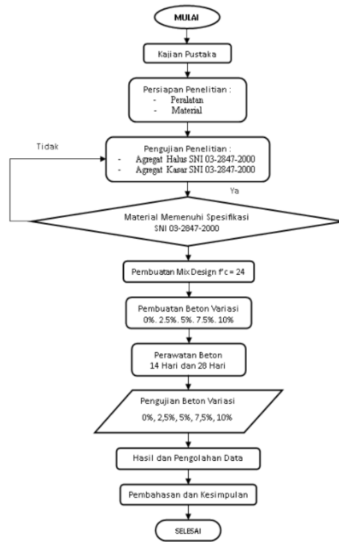
Gambar 1. Flowchart Penelitian 17
