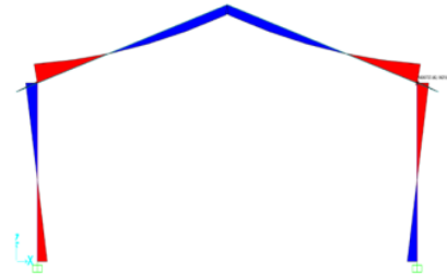
Gambar 9. Diagram Momen
