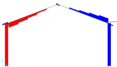
Gambar 8. Diagram gaya geser
