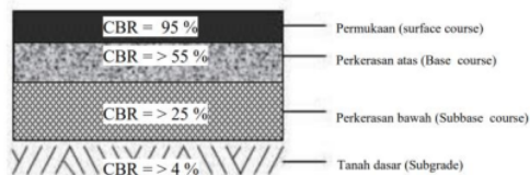
Gambar 8. Lapisan perkerasan lentur ( Unsoaked ) Sumber: A Course in Highway Engineering (S.P. Bindra, 1981)
