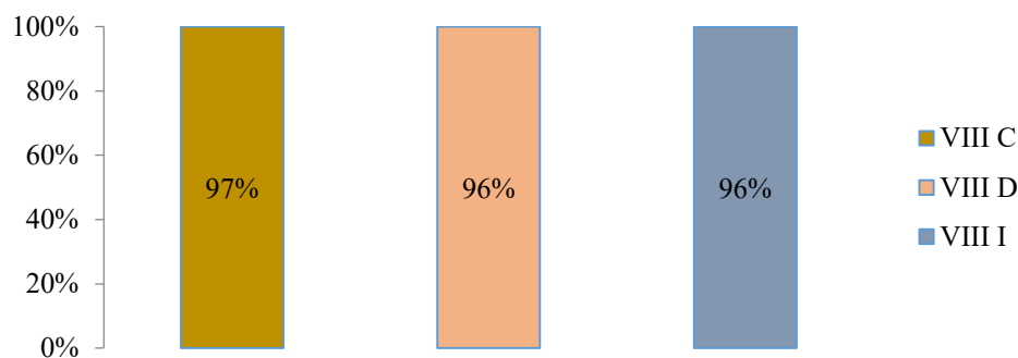
Figure 2. Learning Implementation
