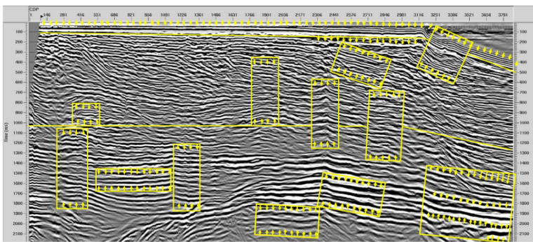
Figure 7. CRS Stack Without Demultiple Noise SMRE and WEMR
