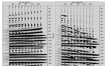
Figure 9. Comparison Radon Analysis Between Signal and Multiple Noise
