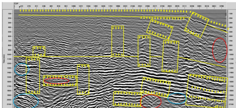
Figure 14. WEMR Output Signal with CRS Stack
