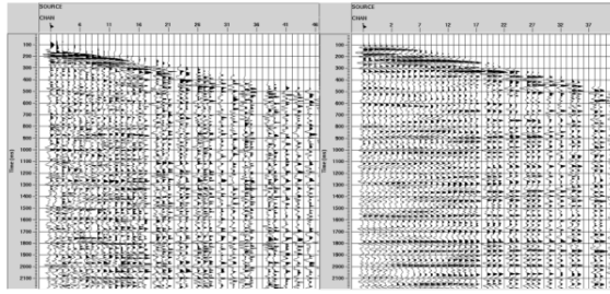
Figure 15. Comparison between multiple noise prediction WEMR (left) and SRME (right)
