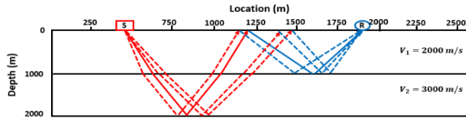
Figure 2. The traces of a common-shot gather in red lines convolving with those of a common receiver gather blue lines predicted Surface multiples. The physical path in solid lines will be obtained and the other contributions will be cancelled by summing all these convolution results
