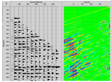
Figure 8. Radon Analysis Lverage to Detect Multiple Noise
