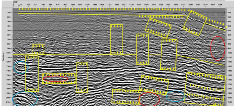
Figure 11. SRME Output Signal with CRS Stack
