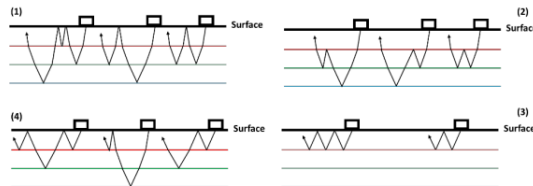
Figure 1. Multiples of Earth or Marine Data: (1) free surface multiple noises (2) inter-bed multiple noises (3) water bottom multiple noises (4) peg-leg multiple noises
