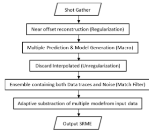
Figure 3. SRME Process Flowchart
