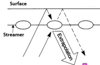
Figure 5. Surface reflected and direct waves interpretation in the wave extrapolation process downward in space and forward in time
