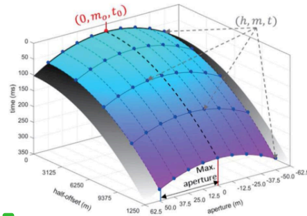
Figure 6. Hyper-Surface of The Two Way Travel Time in CRS Method [40]
