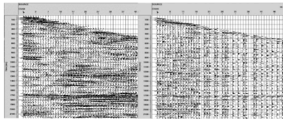
Figure 16. Comparison between SRME and WEMR combine signal (left) and prepro data (right)
