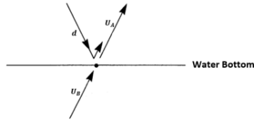
Figure 4. Downgoing and Upgoing Waves Relation at The Water Bottom
