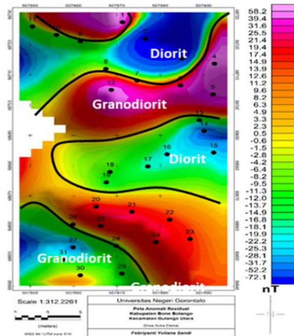
Figure 6. Residual Anomaly Map
