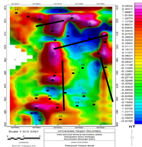
7 Figure 9. Second Vertical Derivative (SVD) Map
