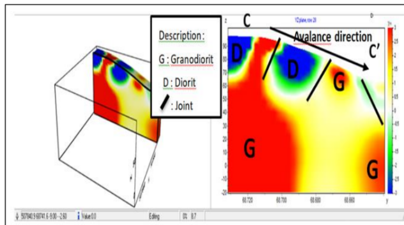
Figure 12. 2D and 3D Modeling (Section C – C')
