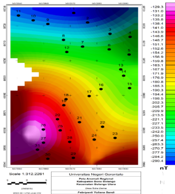
Figure 5. Regional Anomaly Map
