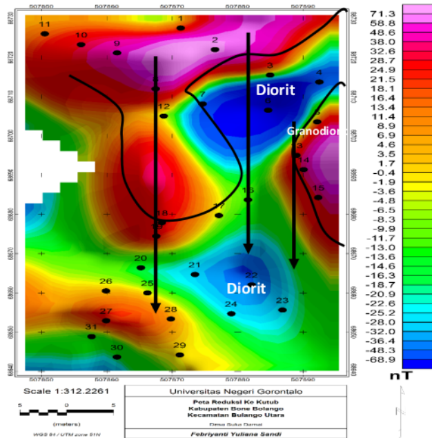
Figure 7. Reduction to the Pole Map
