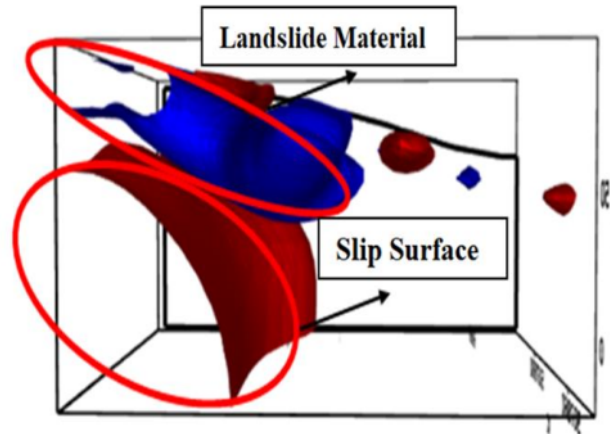
Figure 13. Model 3D Isosurface
