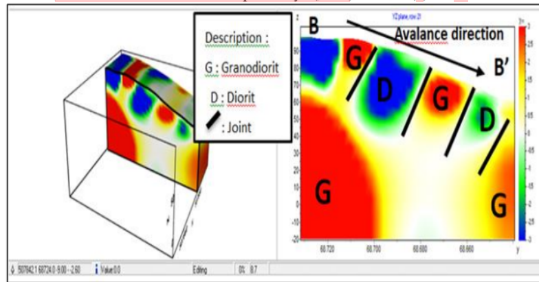
Figure 11. 2D and 3D Modeling (Section B – B')
