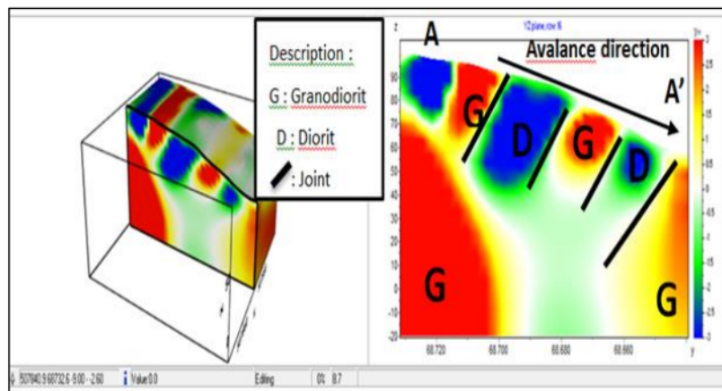
Figure 10. 2D and 3D Modeling (Section A – A')
