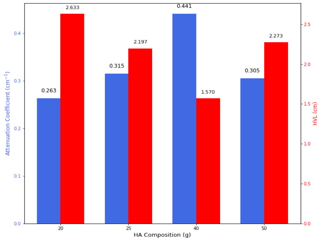
Figure 2. Phantom's linear attenuation coefficient ( \mu ) and HVL.
