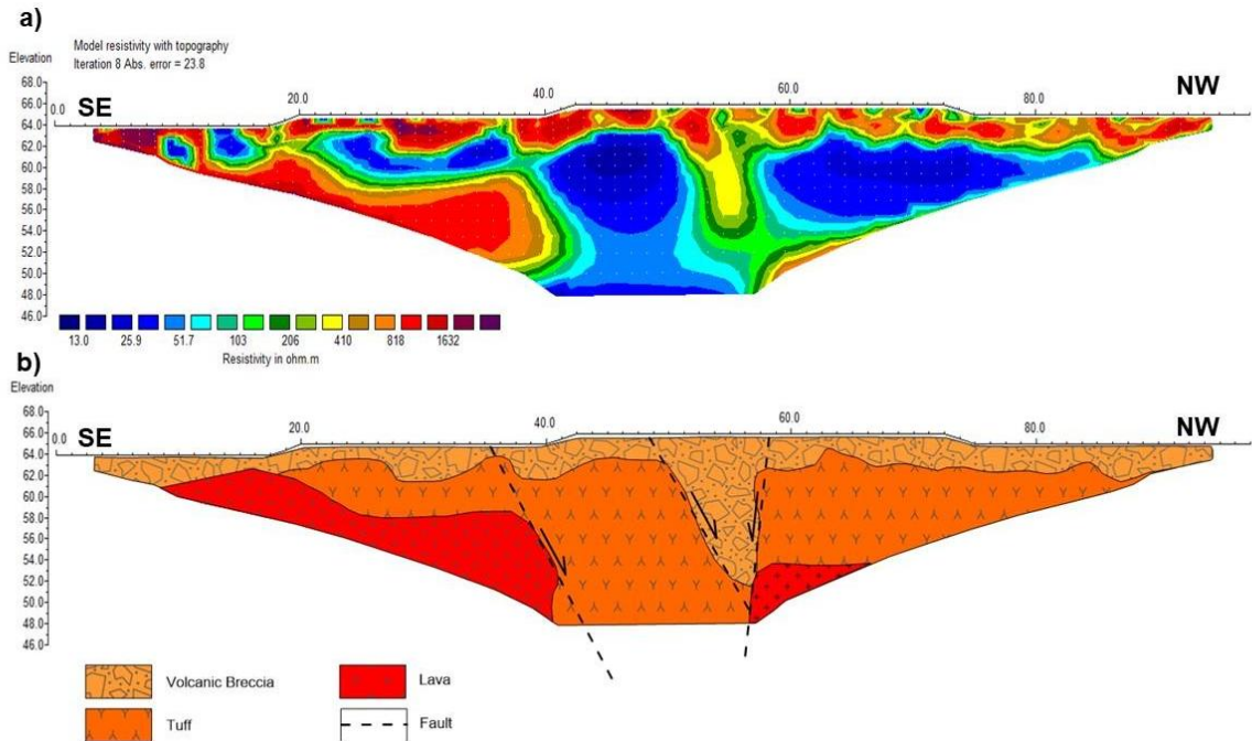
Figure 5. (a) Distribution of subsurface resistivity from inversion modeling, and (b) interpretation of lithology in GL 2.
