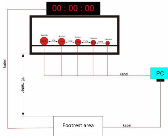
Fig 1. Design of prototype digital slingshot target
