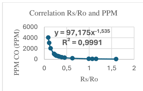
Figure 5. MQ-7 Sensor Characteristic Curve
