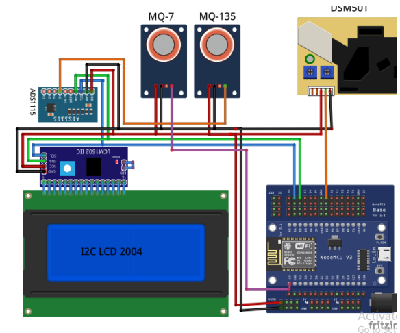
Figure 2. Design Hardware
