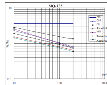
Figure 6. MQ-135 Sensor Characteristics Graph
