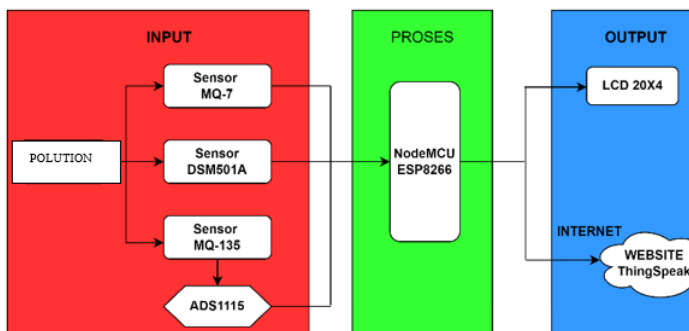
Figure 1. Block Diagram
