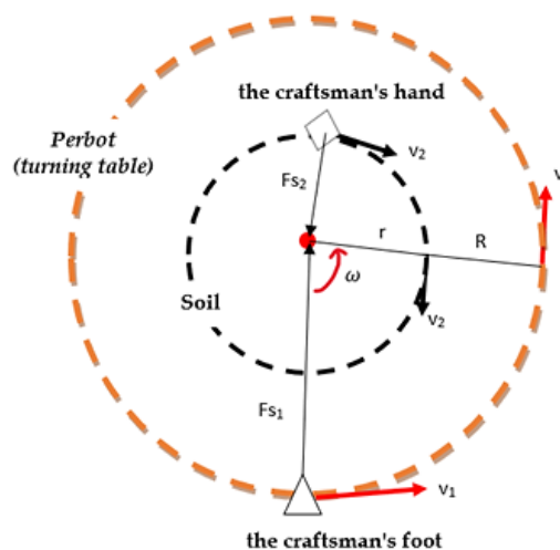
Figure 8. An Illustration of Centripetal Force in the Process of Making cowek with a Lathe (Turntable)
