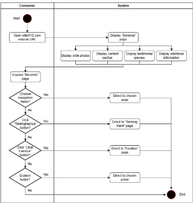
Figure 3. Activity diagram of Beranda page
