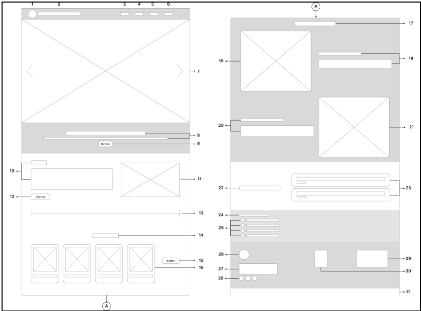
Figure 4. Beranda page wireframe
