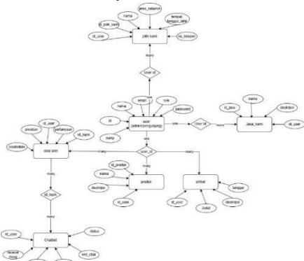
Picture 9 ERD
