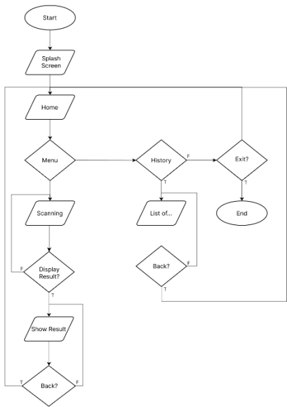
Figure 1 User Flowchart
