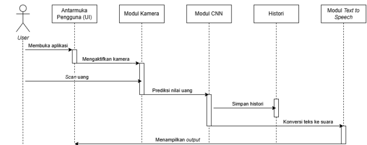
Figure 4 Sequence Diagram
